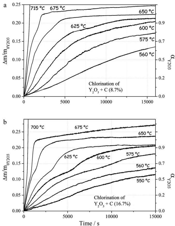
Fig. 7. Effect of temperature on chlorination of Y_2O_3-C (STAGE I). (a) 8.7% C and (b) 16.7% C.
