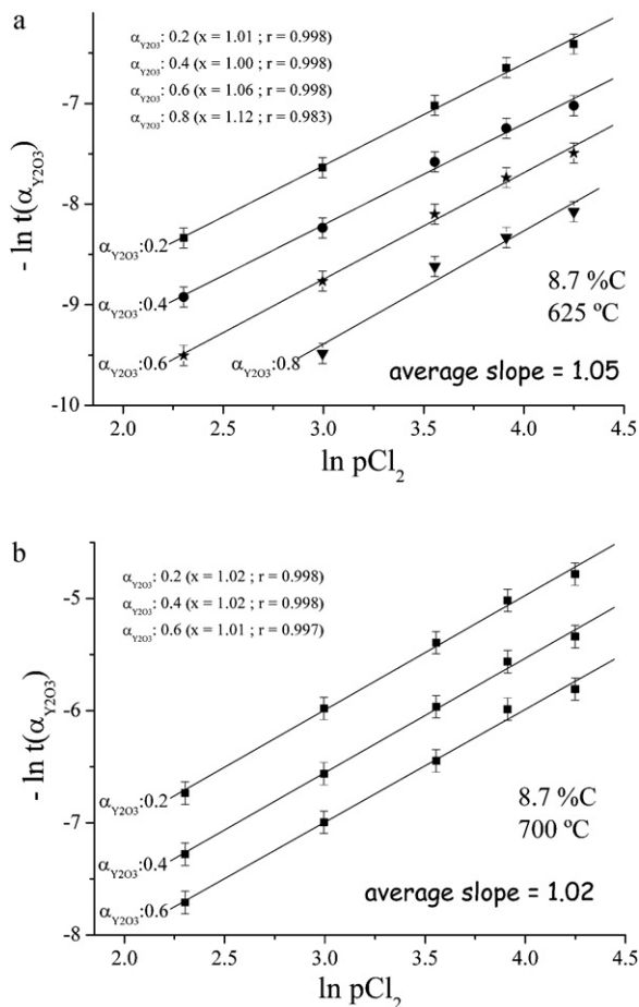
Fig. 6. Plot of Eq. (VIII) at various conversions in the STAGE I. (a) 625 °C and (b) 700 °C.
