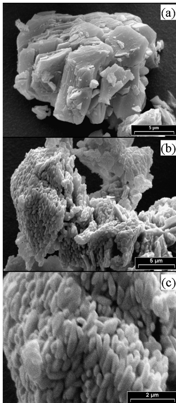
Fig. 9. SEM images of: (a) unreacted Y_2O_3 ; (b) and (c) 675 °C, \alpha_{Y_2O_3} = 1 .
