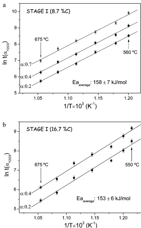
Fig. 8. Plot of \ln t(\alpha) vs. 1/T (Eq. (IX)) at various conversions for STAGE I of Y_2O_3 carbochlorination. The stoichiometry considered corresponds to reaction (1) ( w = 1.16 ). (a) 8.7% C and (b) 16.7% C.
